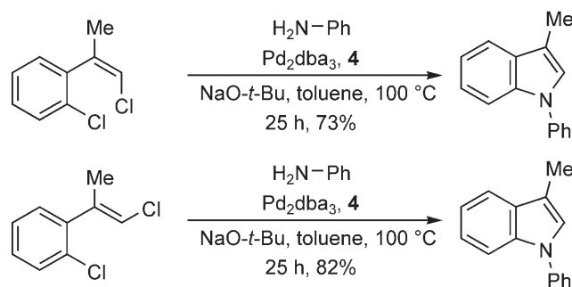
Scheme 2. Utility of E and Z alkenes.
