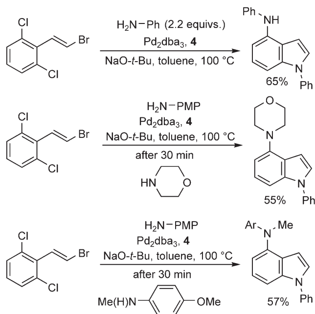
Scheme 3. Sequential amination reactions.
