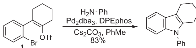
Scheme 1. Tandem Pd-catalysed C–N route in indoles.
